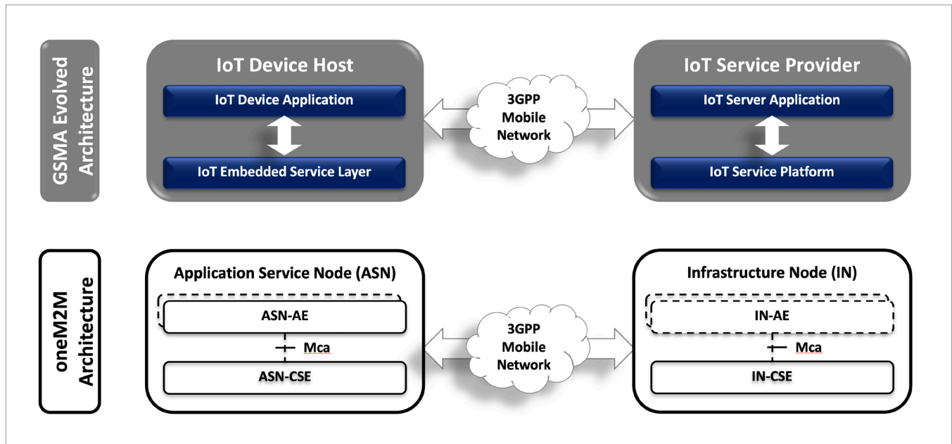
Figure 3- Evolved GSMA Architecture Compared to the oneM2M Standard Architecture
