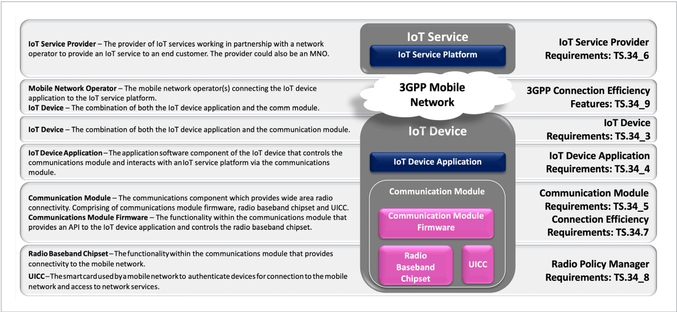
Figure 2 - GSMA Defined IoT Service Architecture
